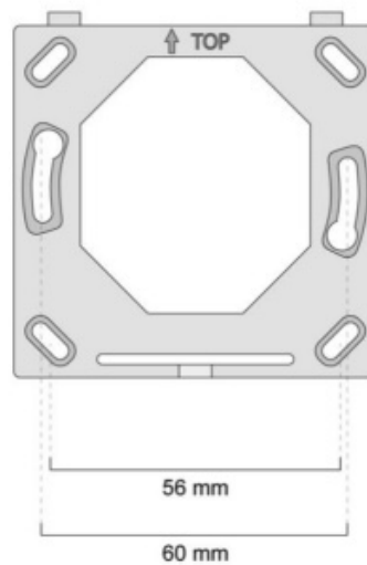
Fig.3. mounting plate
