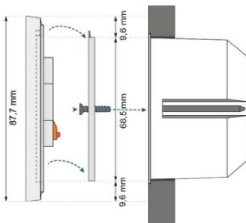
Installation: Touchpanel -> mounting plate -> flush-mounted box
