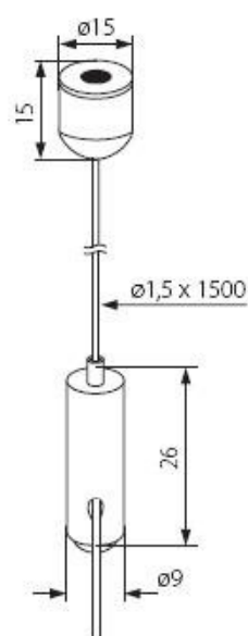
ROPE-NT 150 SINGLE
