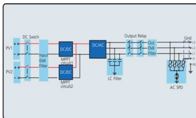
Growatt 3-6kTL3-S topologia
