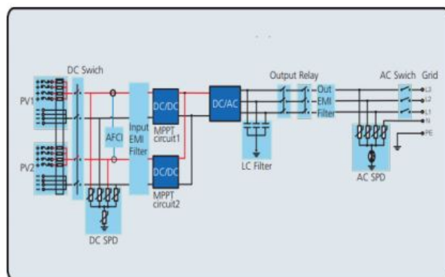
Growatt 17-25kTL3-S topologia
